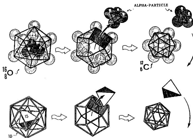
Fig.5. ^{16}\text{O} \rightarrow ^{12}\text{C} + ^4\text{He} The "birth" of a tetrahedron.
