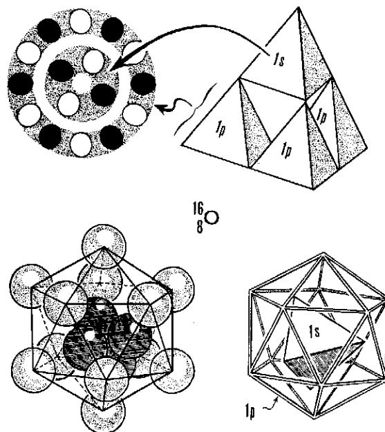
Fig.4. The ^{16}\text{O} nucleus is made from two filled shells. It has a core made from the 1s shell. Its next shell (made from three separate 1p subshells) is made from the three alpha-particles. Generally three tetrahedra, collectively with twelve vertices (nucleons), have no option but to form an icosahedral shell (also with twelve vertices): this is just basic conservation of nucleons! But also it has to do with the fact that the icosahedron has all vertices equally spaced and oriented with respect to each other on the surface of an equivalent sphere. If we were to assume that nucleons are mildly solid spheres which resist compression then this is also a necessary condition for nucleons in a spherical shell. Thus we can abstract the structure of the Oxygen nucleus completely away from the notion of individual nucleons, and instead represent its inner 1s core by a tetrahedron surrounded by an icosahedral shell.
