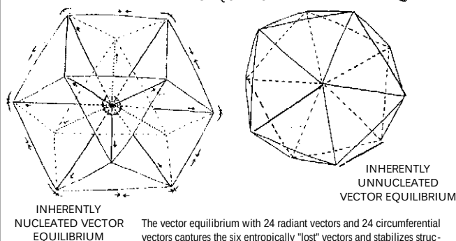
FIG.6 BUCKMINSTER FULLER'S "JITTERBUG" TRANSFORMATION.
