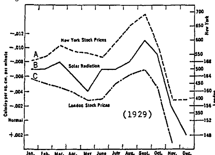
Figure 2. Solar Radiation and Stock Prices
