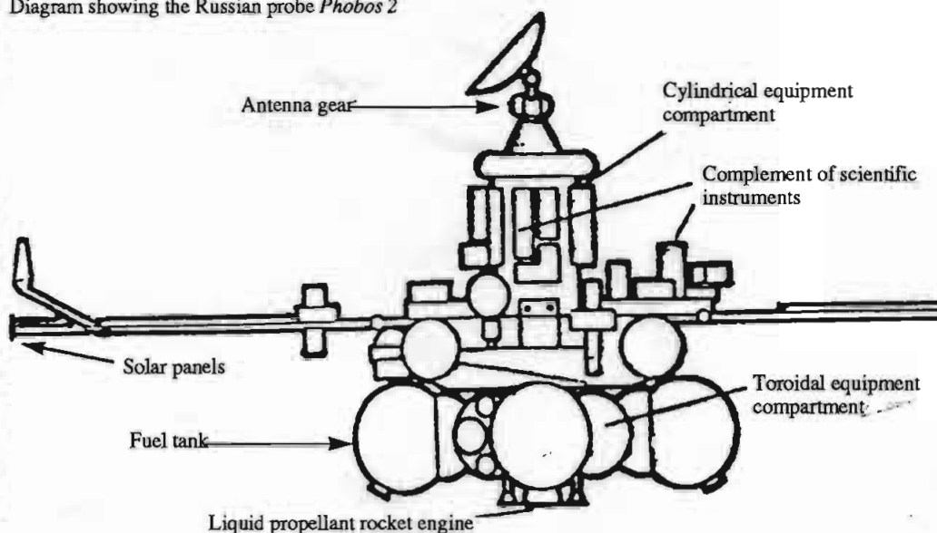
Diagram showing the Russian probe Phobos 2
