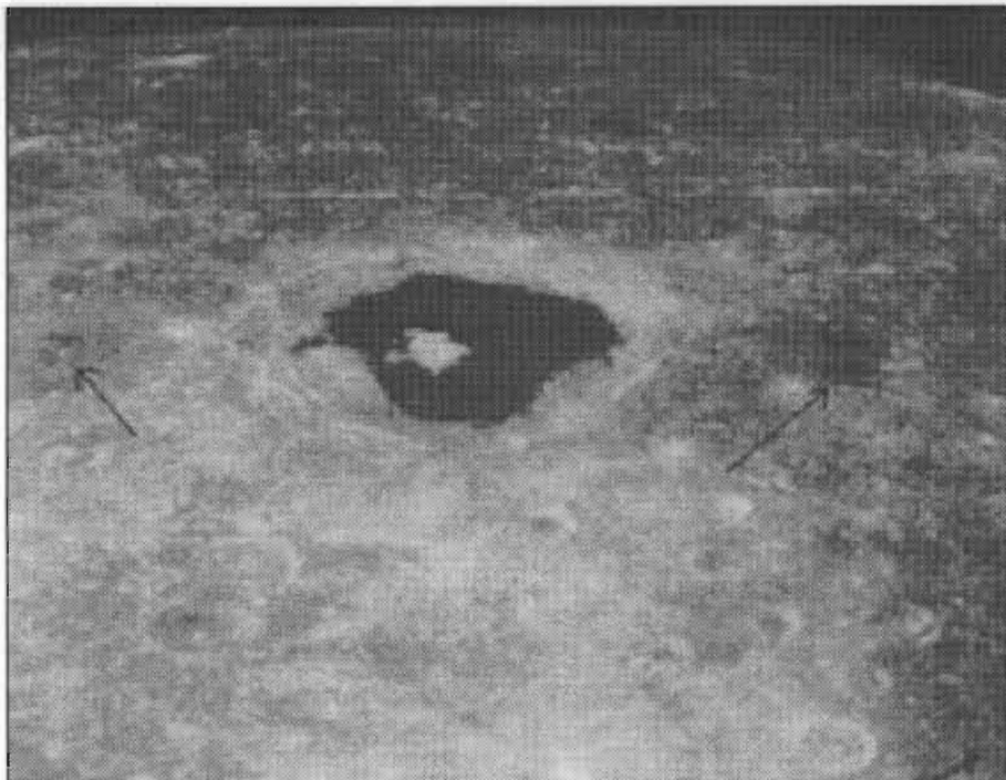
NASA Apollo 8 photograph of the Tsiolkowsky Crater on the dark side of the Moon. Notice the large 'lake' in the centre of the photo and smaller ones on each side.
