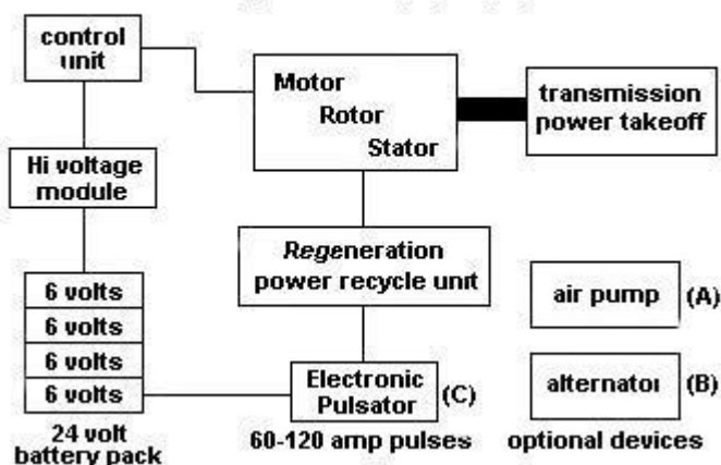
EVGray Motor Block Diagram - 02/25/00 - KeelyNet www.keelynet.com/evgray/evgray.htm
