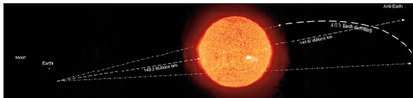
Figure. 2. The Earth–Sun–Counter-Earth system. The invisible area behind the Sun, taking its corona into account, is equal to 10 times the lunar orbit, or 600 times the diameter of the Earth.
