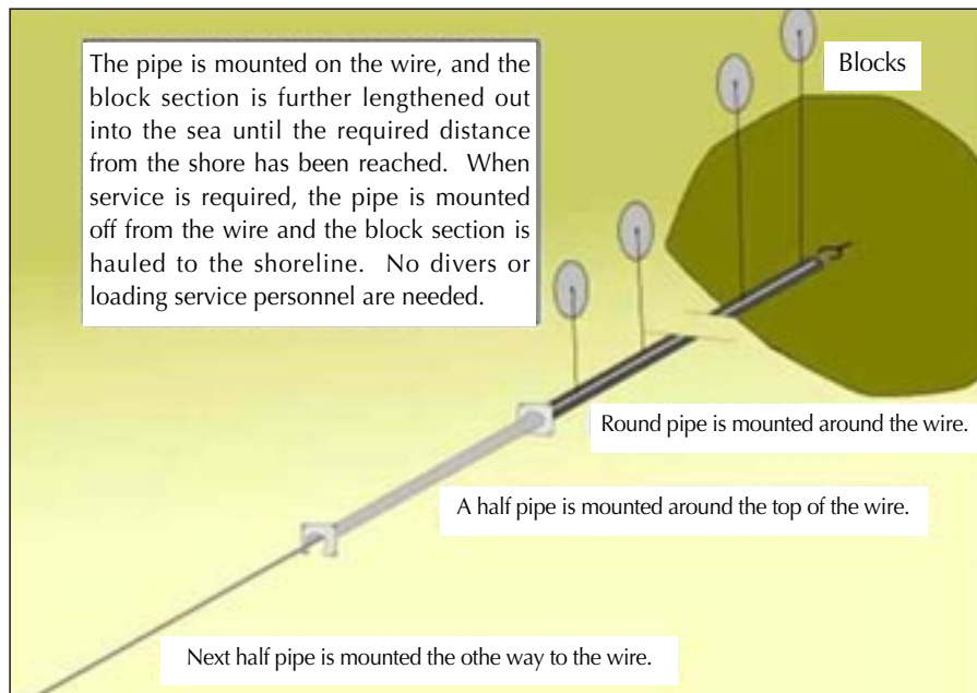
Figure 3. Reverse half-pipe makes it possible to haul gear without divers. The pipe is mounted on the wire, and the block section is further lengthened out into the sea until the required distance from the shore has been reached. When service is required, the pipe is mounted off from the wire and the block section is hauled to the shoreline. No divers or loading service personnel are needed. Round pipe is mounted around the wire. A half-pipe is mounted around the top of the wire. The next half-pipe is mounted the other way to the wire.
