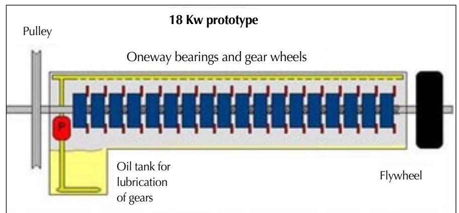
Figure 5. Schematic of 18 kW WaveReaper™ prototype.
